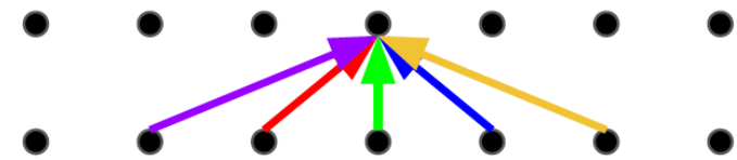
Self-Attention
