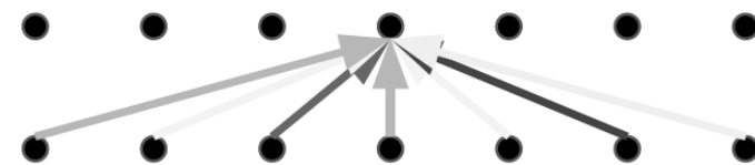
Multi-Head Attention
